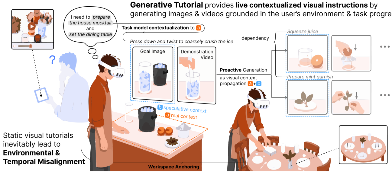
Figure 1: Generative Tutorial reimagines tutorials as live, contextualized visual instructions adapted to a user’s environment and evolving task progress. The prototype system continuously captures real-world context and grounds the task model in the user’s environment. For each step, it aims to generate a workspace-grounded goal image and demonstration video (e.g., showing how to press and twist a muddler to crush ice). By propagating real and speculative visual context forward, the system proactively generates guidance for upcoming steps (e.g., squeezing juice and preparing a mint garnish). The generated guidance is presented and situated in its associated task workspace, allowing instructions to coexist across activities and remain available as the user switches between them (e.g., moving from preparing a house mocktail to setting the dining table).
