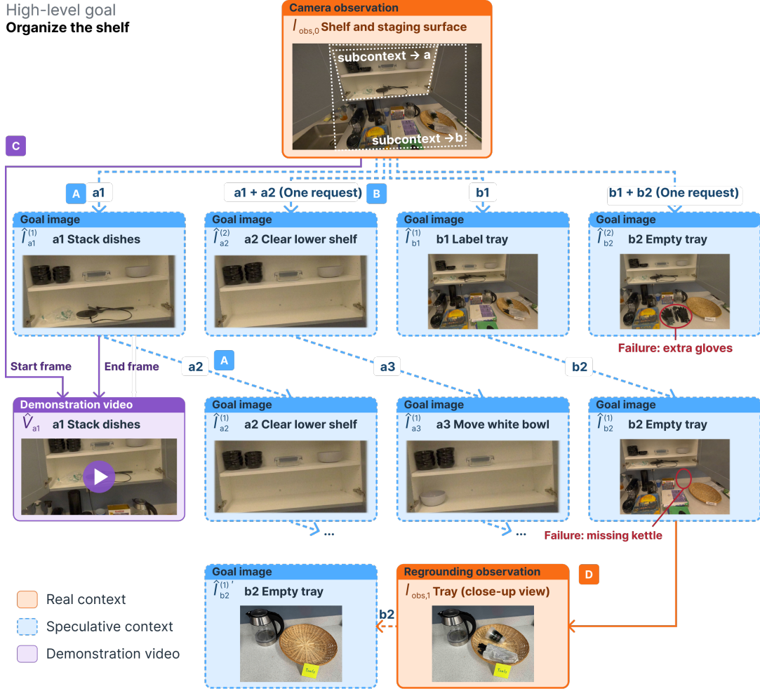
Figure 6: Visual state propagation illustrated through shelf organizing. Orange denotes camera observations (real context), blue predicted outcomes (speculative context), and purple demonstration video. The initial observation contains two workspace-specific subcontexts: the shelf ( a ) and the staging surface containing the tray ( b ). (A) Sequential prediction uses each predicted outcome as the next action’s source. (B) Two-action prediction generates the combined outcome in one request, providing an alternative route to the same intended state. (C) Video generation uses source and predicted outcome images as start and end frames. (D) Regrounding replaces speculative context with a fresh observation. Red annotations mark observed errors, not automatic detection.
