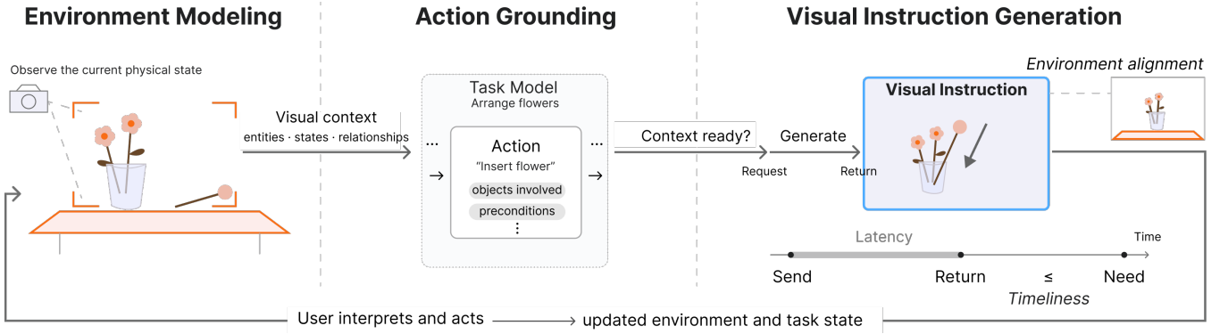
Figure 2: Conceptual framework for Generative Tutorial, illustrated through flower arranging. Environment Modeling represents observed entities, states, and relationships as visual context. Action Grounding relates an action in the task model, including its objects and preconditions, to the current scene. Once sufficient context is available, Visual Instruction Generation depicts how to act or what the action should achieve. Environment alignment connects the depiction to the physical scene, while timeliness concerns its availability at the time of need. User interpretation and action lead to changes in the environment and task state that inform subsequent guidance.
